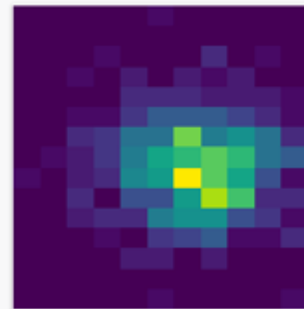
2d-histogram
