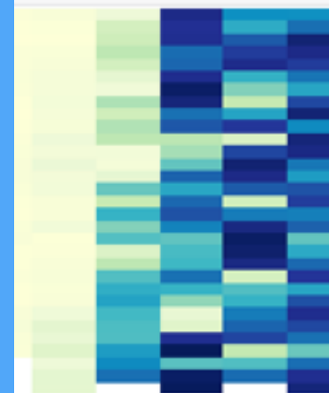
posts-per-day
